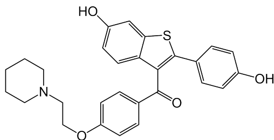
Raloxifene Structure (C 28 H 27 NO 4 S; MW: 473.2)
