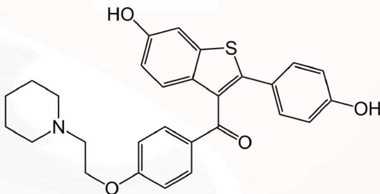
Raloxifene Structure (C 28 H 27 NO 4 S; MW: 473.2)
