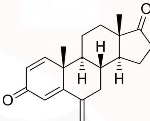
Aromasin Exemestane Structure
