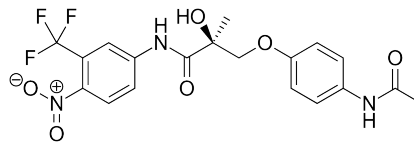
Andarine (S4) Structure (C 19 H 18 F 3 N 3 O 6 MW: 441.12; m/z: [M+H] 442.1099)
