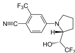
LGD4033 Structure (MW: 338.226)
